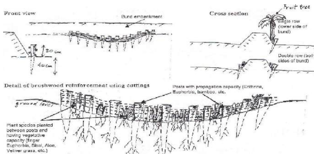
Figure 3: Reinforcing bunds along depression points Source: http://www.fao.org .
