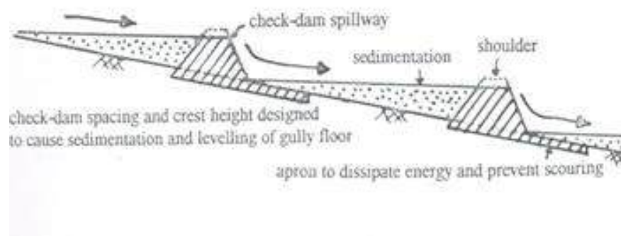
Figure 3: Determination of check dams spacing and the layout Source: http://www.fao.org
