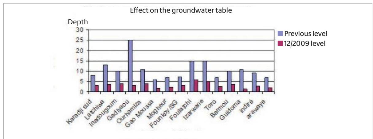
Figure 11: Rise of the groundwater table in rehabilitated valleys in Niger. Source: Sulser, p. 9, according to Betifor (2010)
