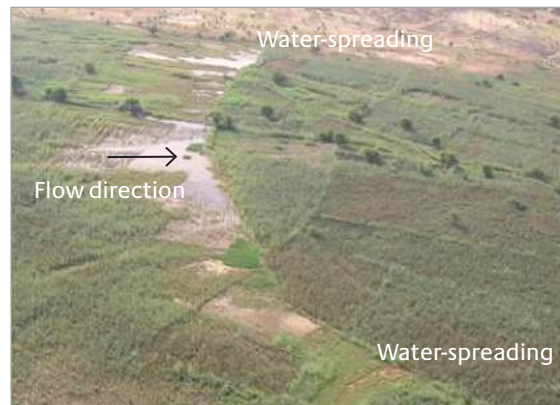
Figure 12: The water is distributed over the entire width of the water-spreading weir, resulting in more infiltration above and below. As a result crops can be grown (in this case sorghum and some rice) over the entire width of the valley floor above and below the weir. Source: Bender (2011)
